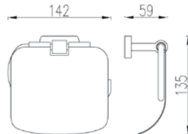
LovA Paper Holder - Elegance BPH031
