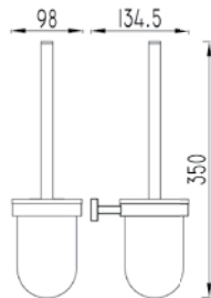
LovA Elegance HOSPTBW7 Extra brushes in option
