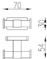
LovA Double Hook - Elegance BH032
