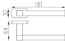
LovA Paper Holder - Elegance BPH032
