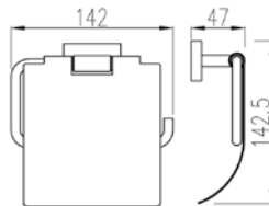
LovA Paper Holder - Quadra BPH021
